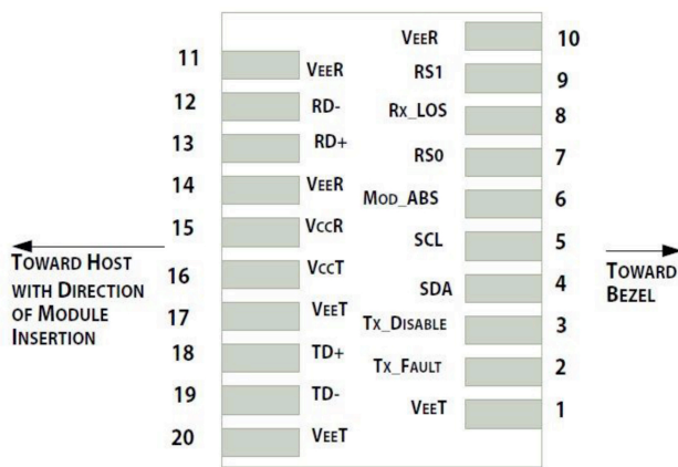
Pin-out of connector Block on Host board
