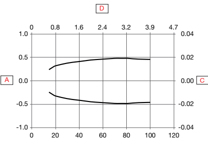
Fig. 5 Precise mode
