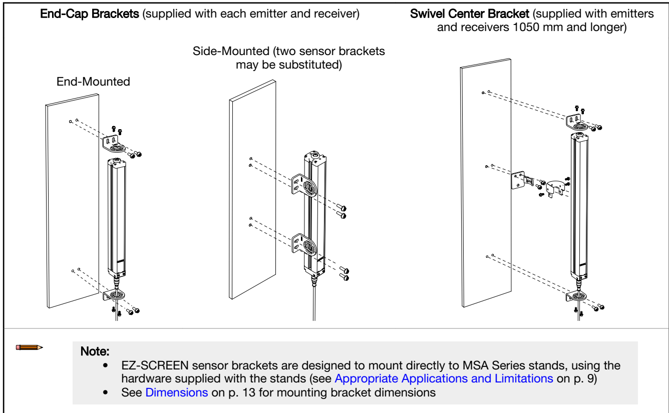
Figure 10. Sensor Brackets
