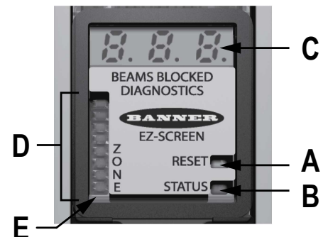
Figure 26. Receiver
