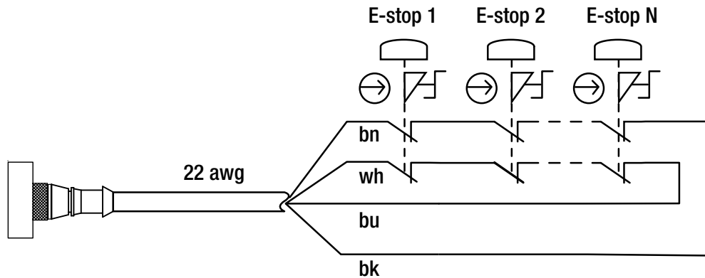
Figure 28. Wiring of emergency stop buttons to the last receiver in the cascade.
